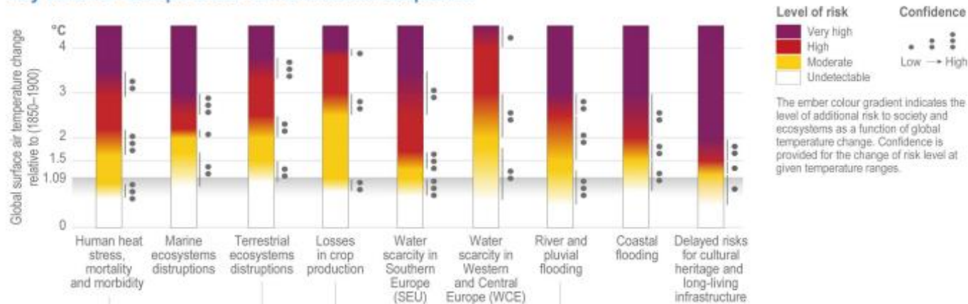
Key risks for Europe under low to medium adaptation
